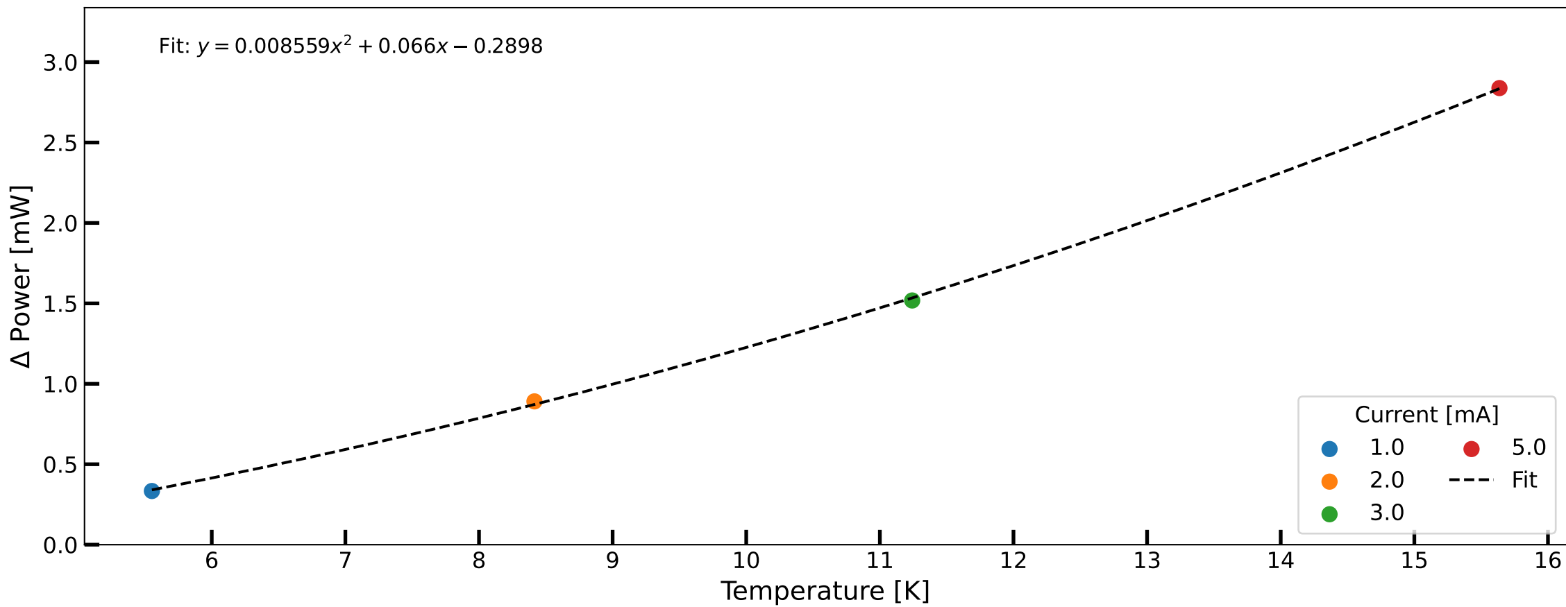
Coarse: Power Difference (Measured - I^2 1k\Omega )
