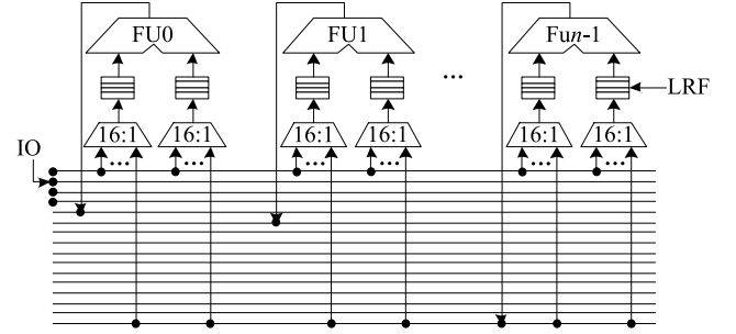
FIGURE 3. Structure of stream processor.
