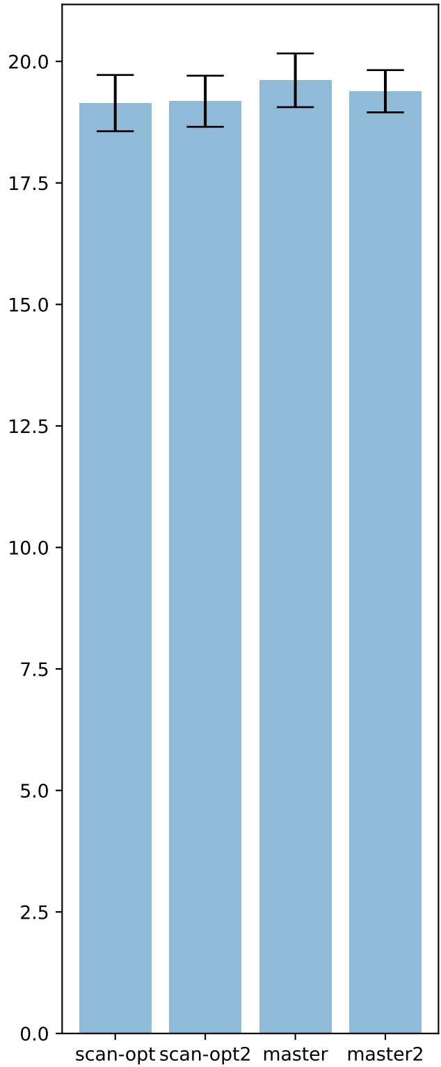
Execution Time
