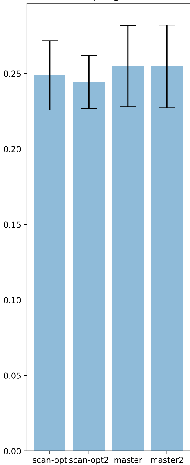
Compiling Time
