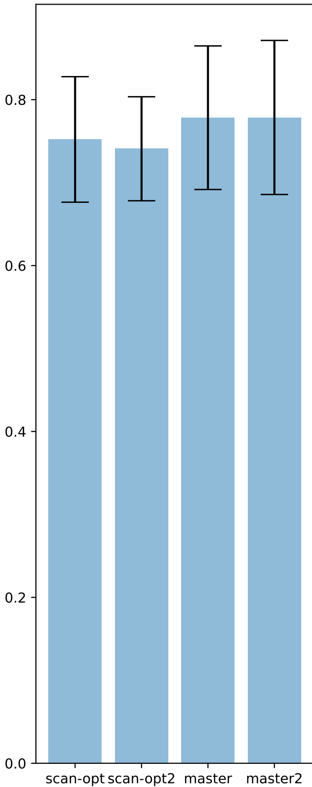
Compiling Time
