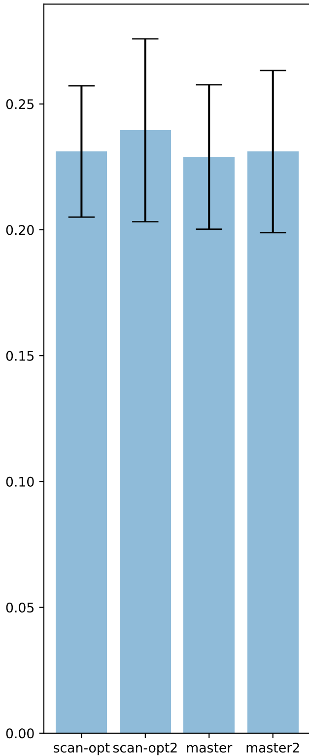
Compiling Time
