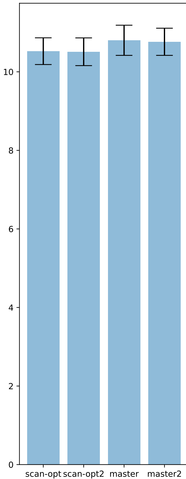
Execution Time
