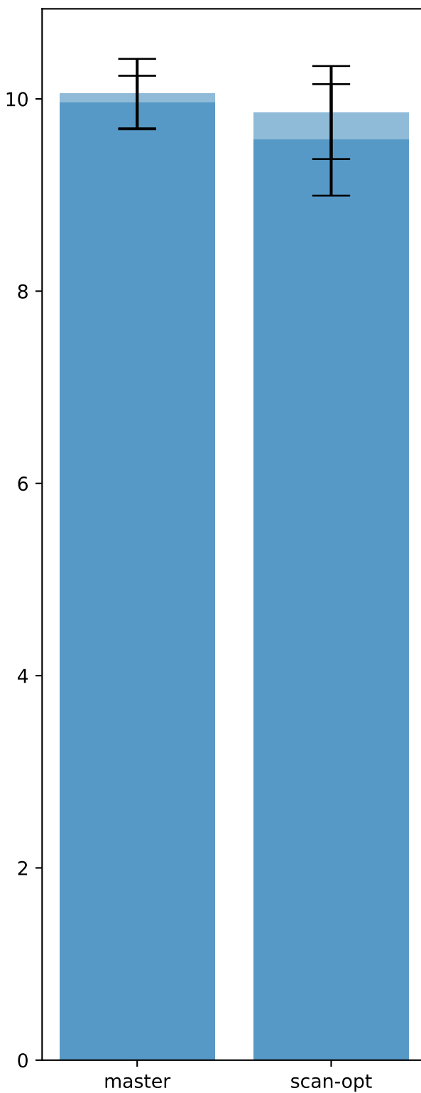
Execution Time
