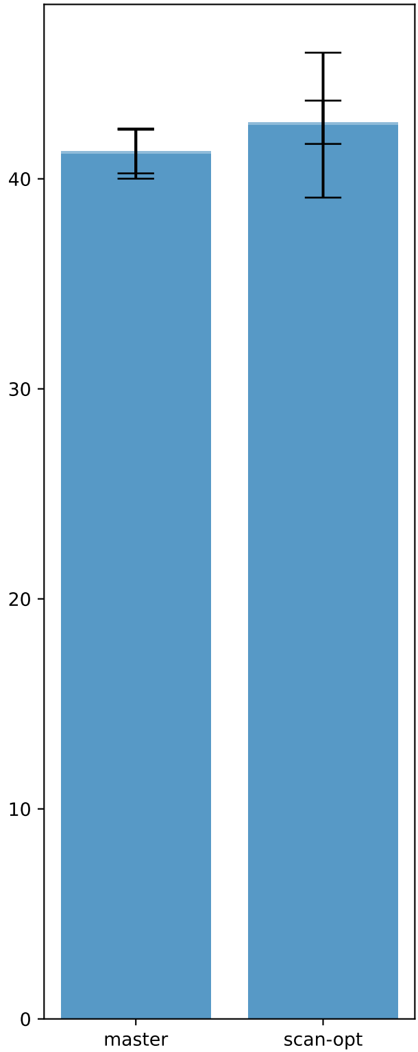
Execution Time
