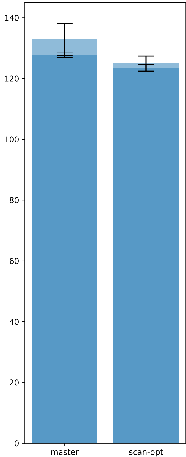
Execution Time
