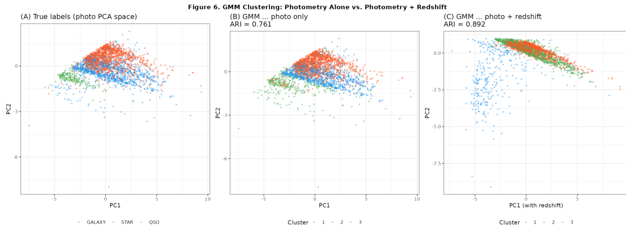
Figure 6: GMM clustering: photometry alone vs. photometry + redshift. (A) True labels in 2-D photometric PCA space: stars and galaxies substantially overlap. (B) GMM with 3 components on photometric features: \text{ARI} = 0.76 , reflecting poor recovery of the true class structure. (C) Adding redshift as a feature produces near-perfect cluster recovery ( \text{ARI} = 0.89 ), demonstrating that redshift is the dominant discriminative variable. All panels show 3,000 random objects.
