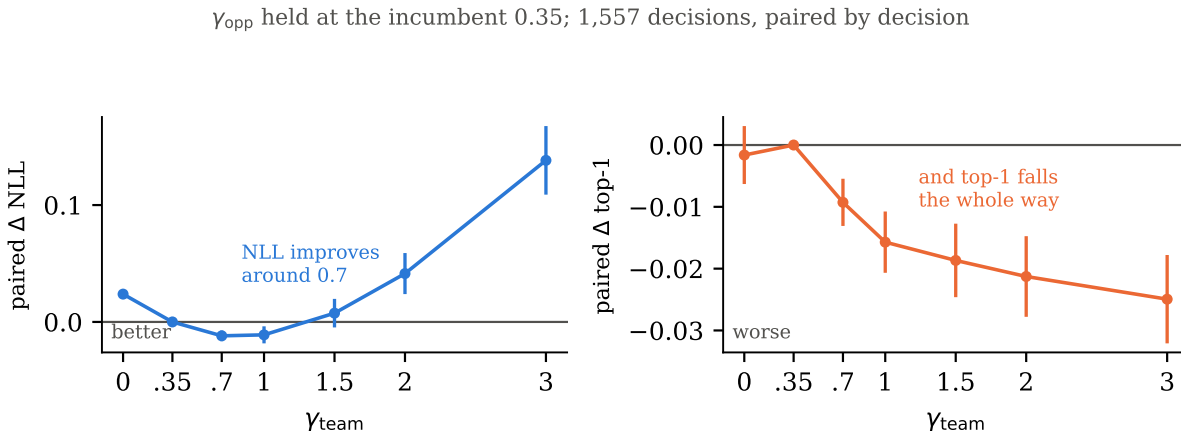
Figure 8: Why the teammate-side model was withdrawn. Both panels are paired against the incumbent cell by decision — cards inside one decision share a belief, so the card is not the independent unit — with \gamma_{\text{opp}} held at the shipped 0.35. Sharpening the model on our own side buys a small improvement in the proper score around \gamma_{\text{team}} = 0.7 and pays for it by naming the true holder less often at every setting. The allocation decision reads the argmax, so that is a worse belief for the job it has to do.
