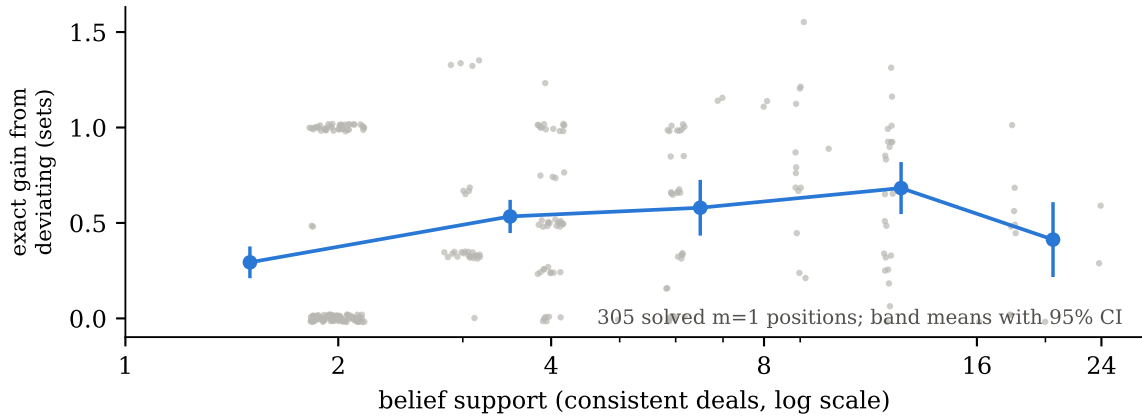
Figure 6: What an exact deviation is worth, against how much the belief leaves open, over the 305 solved m = 1 positions. Gray points are positions (jittered for visibility); blue points are means over support bands with 95% confidence intervals. The gain rises with support — and the unsolved positions lie beyond the right edge of this plot, at a median support of 48 against a solved median of 3. That is why the solved-layer means read as lower bounds, why §24.4 tries to replace that extrapolation with bounds, and why the honest answer is that the plot cannot be read past its own right edge.
