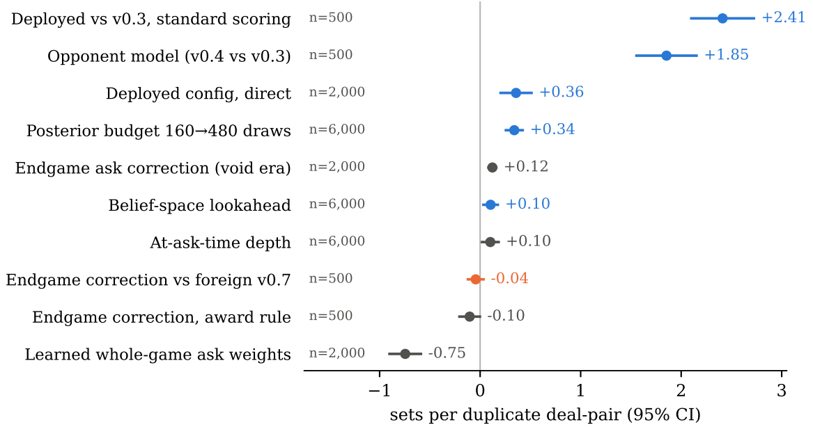
Figure 2: Every settled in-play effect, on one axis. Blue rows ship in the deployed configuration; gray rows were evaluated and not shipped — at-ask-time depth a null at n = 6000 , the learned whole-game weights significantly worse, and the endgame ask correction shipped in the void era and withdrawn when the award baseline re-priced it below zero (§27). The orange row is that correction against a foreign engine, Dylan’s FishBot v0.7, under the matched award rule: a tie whose interval excludes the sibling-measured void-era +0.12 — the paper’s recurring finding that gains measured inside an engine family shrink outside it. Intervals are 95% confidence intervals over paired deals; n counts pairs.
