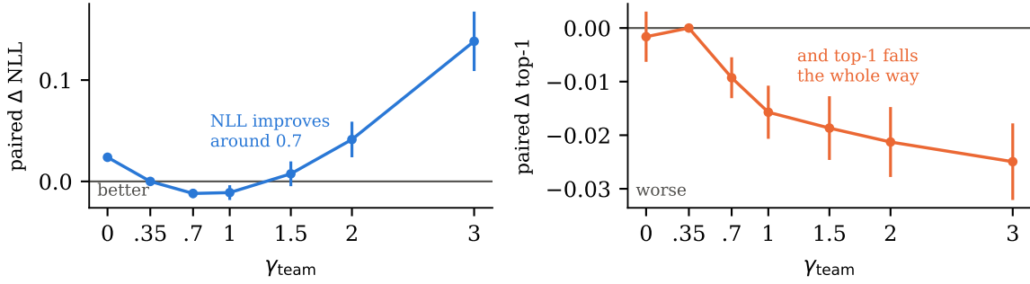
Figure 8: Why the teammate-side model was withdrawn. Both panels are paired against the incumbent cell by decision — cards inside one decision share a belief, so the card is not the independent unit — with \gamma_{\text{opp}} held at the shipped 0.35. Sharpening the model on our own side buys a small improvement in the proper score around \gamma_{\text{team}} = 0.7 and pays for it by naming the true holder less often at every setting. The allocation decision reads the argmax, so that is a worse belief for the job it has to do.
