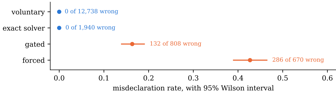
Figure 4: Every misdeclaration this engine makes is compelled. Split by the path the declaration arrived on: the two paths it takes because it wants to be exactly perfect over 14,678 declarations between them, and both paths where it declares because it must — the endgame gate, and a forced declaration with no cards left to ask with — carry the whole error rate. This is why the headroom in §16 is not a calibration problem. The policy already declines every declaration it is entitled to decline.
