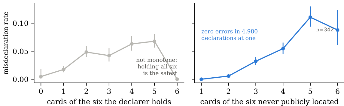
Figure 3: The lever everyone reaches for, and the one that carries the risk. Left: misdeclaration rate against how many of the six the declarer holds. It is not even monotone — holding all six is the safest state there is, so the curve turns over at the right-hand end, and any policy tuned on this covariate is tuned on a confound. Right: the same declarations against how many of the six have never been publicly located . That one runs from zero errors in 4,980 declarations up to eleven percent. The dip at six is 30 errors in 342 declarations and its interval covers the point before it. Bars are 95% Wilson intervals, which is why the zero cell has a visible upper limit rather than a degenerate one.
