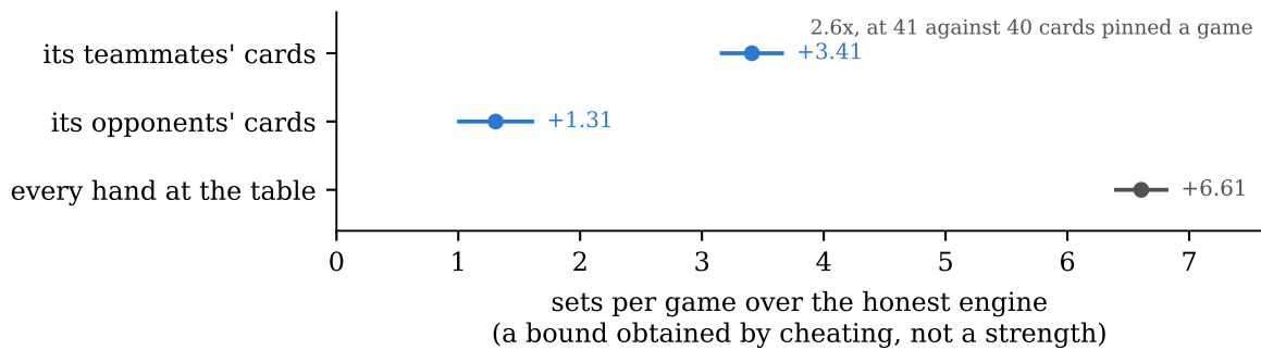
Figure 5: What perfect card-reading is worth, one side of the table at a time. Every value here is obtained by cheating: the arm is handed the true deal and the opposition never is, so these bound what information could buy and are not strength measurements. They never appear in a ladder. The two partial arms are told almost exactly the same number of cards — 40.7 against 40.4 a game — and the teammate side is worth 2.6× the opponent side anyway. We predicted the reverse. The two do not sum to the whole (4.72 against 6.61), so the sides are complements rather than separable contributions.
