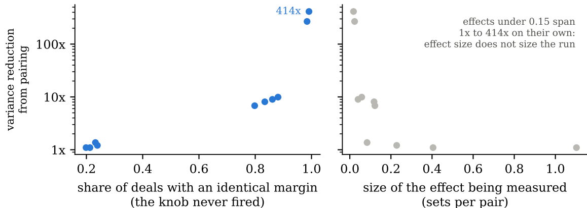
Figure 1: What actually sizes a duplicate-deal run. Left: the variance-reduction factor from pairing against the share of deals on which both arms produced an identical margin — that is, on which the knob under test never changed a decision. The relationship is tight over more than two orders of magnitude. Right: the same factor against the size of the effect being measured, which is the quantity everyone reaches for when planning a run and which does not determine the answer: effects below 0.15 sets per pair span the entire range on their own. Same runs as Table 2.
