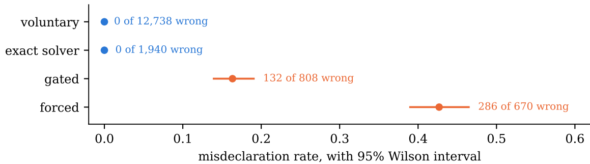
Figure 3: Every misdeclaration this engine makes is compelled. Split by the path the declaration arrived on: the two paths it takes because it wants to be exactly perfect over 14,678 declarations between them, and both paths where it declares because it must — the endgame gate, and a forced declaration with no cards left to ask with — carry the whole error rate. This is why the headroom in §16 is not a calibration problem. The policy already declines every declaration it is entitled to decline.
