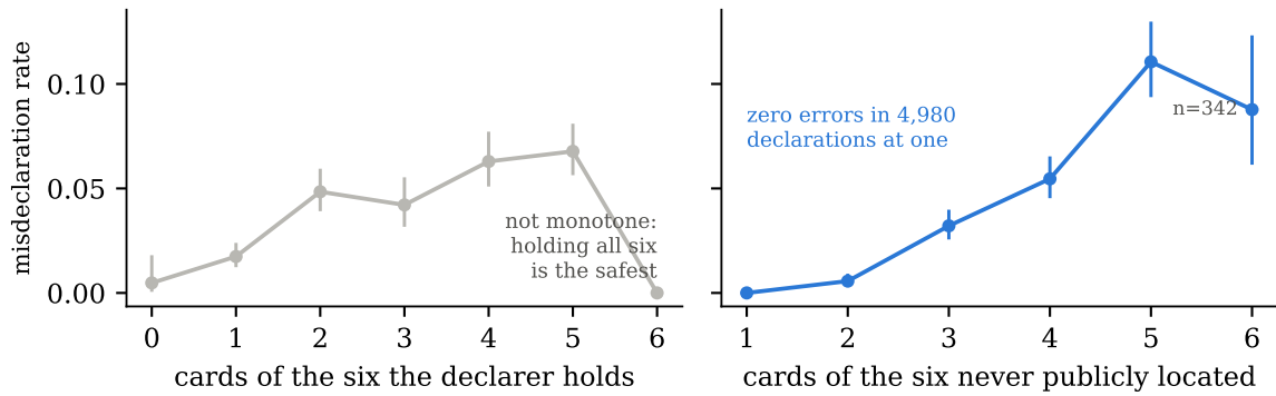
Figure 2: The lever everyone reaches for, and the one that carries the risk. Left: misdeclaration rate against how many of the six the declarer holds. It is not even monotone — holding all six is the safest state there is, so the curve turns over at the right-hand end, and any policy tuned on this covariate is tuned on a confound. Right: the same declarations against how many of the six have never been publicly located . That one runs from zero errors in 4,980 declarations up to eleven percent. The dip at six is 30 errors in 342 declarations and its interval covers the point before it. Bars are 95% Wilson intervals, which is why the zero cell has a visible upper limit rather than a degenerate one.
