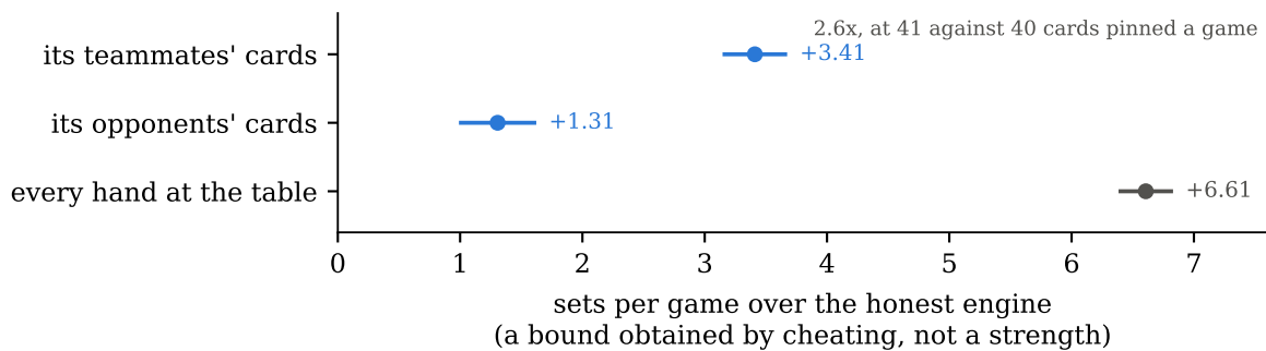
Figure 4: What perfect card-reading is worth, one side of the table at a time. Every value here is obtained by cheating: the arm is handed the true deal and the opposition never is, so these bound what information could buy and are not strength measurements. They never appear in a ladder. The two partial arms are told almost exactly the same number of cards — 40.7 against 40.4 a game — and the teammate side is worth 2.6× the opponent side anyway. We predicted the reverse. The two do not sum to the whole (4.72 against 6.61), so the sides are complements rather than separable contributions.
