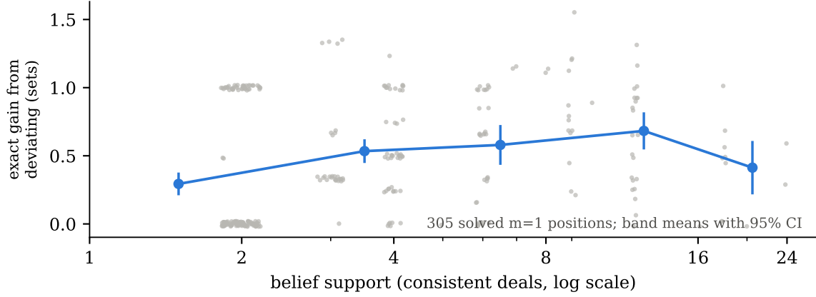
Figure 5: What an exact deviation is worth, against how much the belief leaves open, over the 305 solved m = 1 positions. Gray points are positions (jittered for visibility); blue points are means over support bands with 95% confidence intervals. The gain rises with support — and the unsolved positions lie beyond the right edge of this plot, at a median support of 48 against a solved median of 3. That is why the solved-layer means read as lower bounds, why §24.4 tries to replace that extrapolation with bounds, and why the honest answer is that the plot cannot be read past its own right edge.
