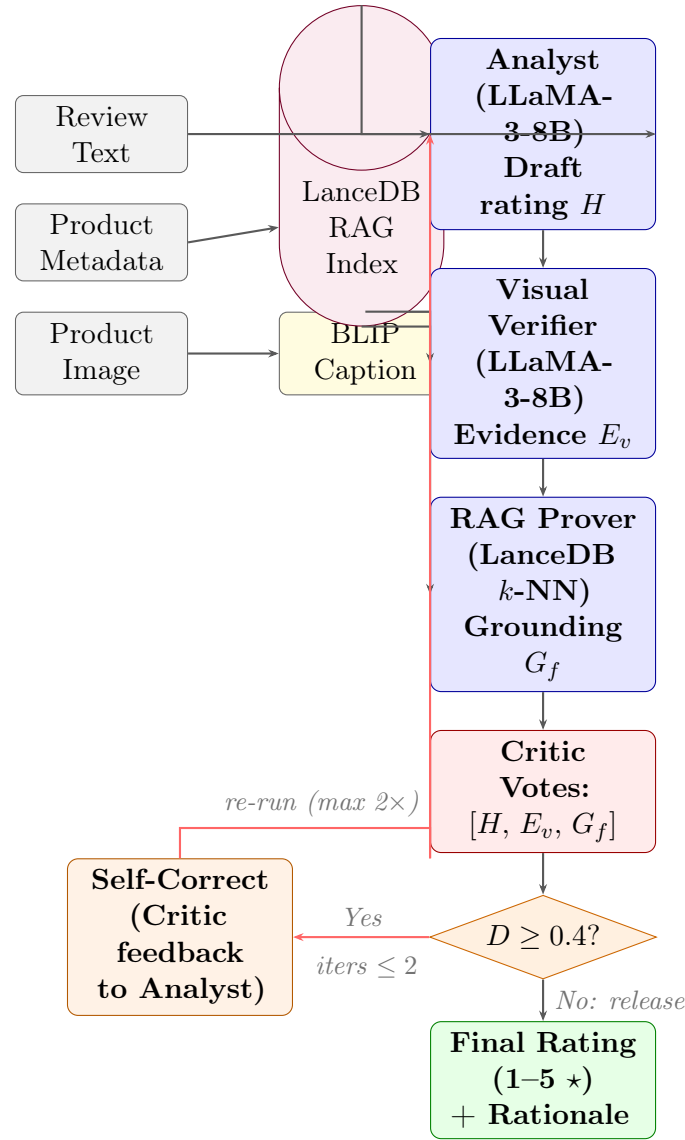
Figure 2: Phase 2 multi-agent pipeline. Review text, product metadata, and BLIP image captions feed three specialised agents. The Critic computes dissonance D from the agent votes; if D \geq 0.4 , a self-correction loop sends critique feedback back to the Analyst (up to 2 iterations). Otherwise the majority-vote rating and rationale are released.
