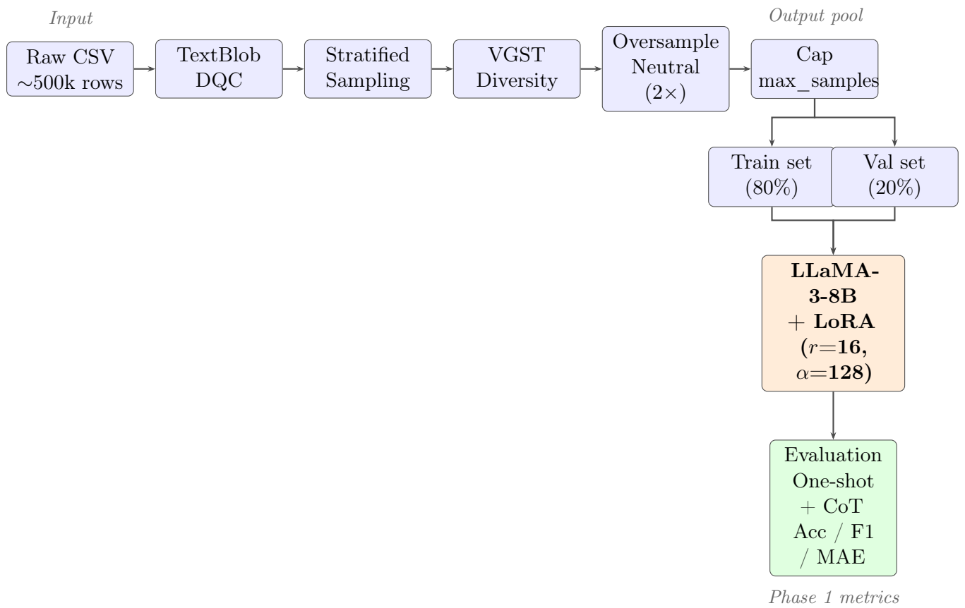
Figure 1: Phase 1 end-to-end data and training flow. Raw CSV reviews pass through five preprocessing stages before being split into train/val. LLaMA-3-8B with LoRA is fine-tuned on the training set; evaluation uses one-shot + CoT prompting.
