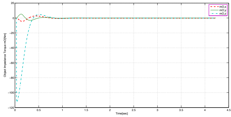
Figure 4.7: Impedance torque m_O during rotation about the z axis (rotation 0.6 rad).
