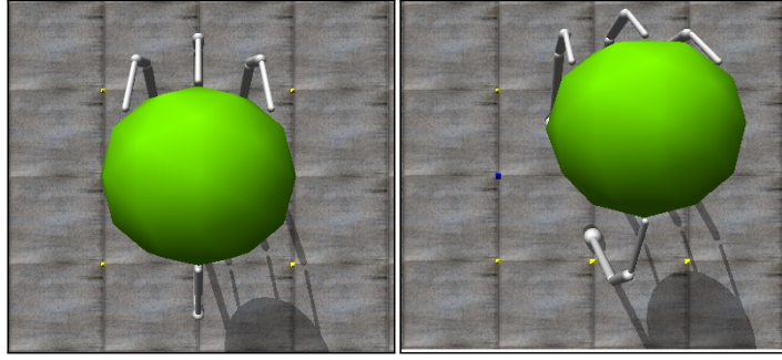
Figure 4.6: Top view – displacement along the x_o axis (translation 40 cm).
