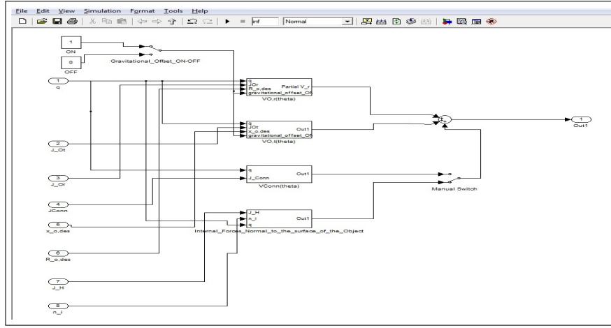
Figure 4.3: View of the Simulink internal stiffness terms (rotational and translational).
