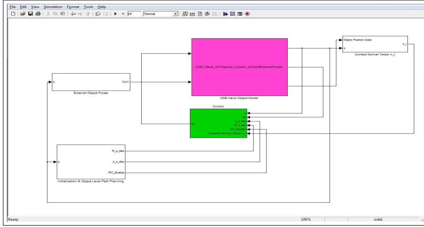
Figure 4.1: Top-level Simulink implementation view including the system model, the controller, and the auxiliary tools.
