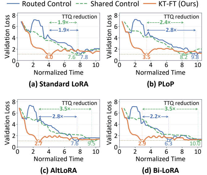
Figure 11. Loss convergence of KT-FT (Ours) and the two controls across LoRA variants.
