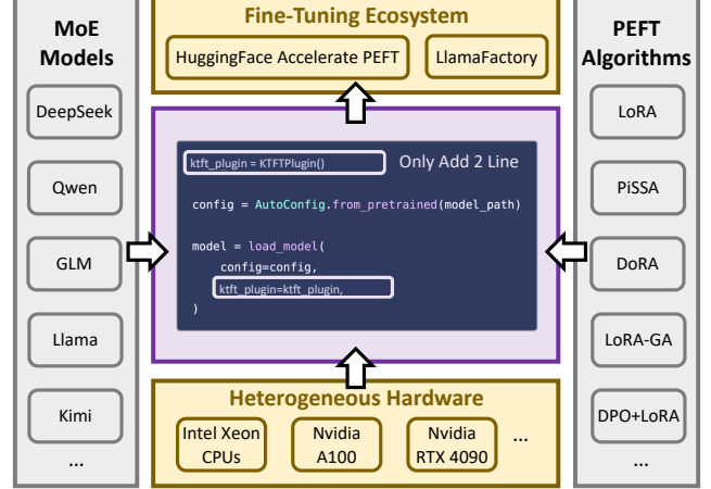
Figure 4. KT-FT’s integration with the fine-tuning ecosystem.
