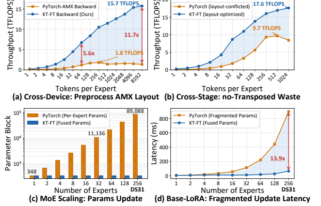
Figure 2. Memory layout conflicts and their effects on MoE fine-tuning. Panel (a) reports end-to-end MoE backward-pass throughput under the cross-device layout requirement, while panel (b) reports expert GEMM throughput under the cross-stage layout requirement; panels (c) and (d) report parameter block counts and optimizer step latency for fragmented and fused LoRA parameter layouts. All measurements use a DeepSeek-V3.1 (DS31) configuration representative of trillion-parameter MoE models.
