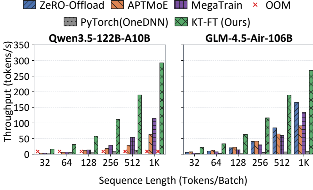
Figure 9. Full-parameter fine-tuning on Single-Node.
