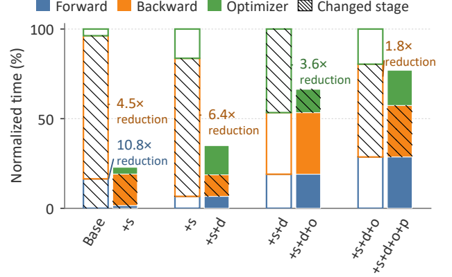
Figure 10. DS-31 LoRA ablation. Each pair shows the previous (unfilled) and current (filled) configurations, with times normalized to the previous configuration’s total step time. Numbers denote stage time reduction factors. Base is PyTorch(OneDNN), and the final configuration is KT-FT (Ours).
