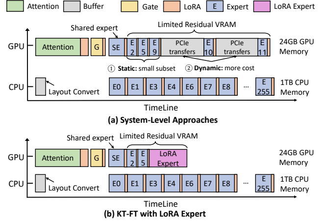
Figure 7. Allocation of residual VRAM. A small subset of hot experts is statically cached, and the remaining capacity is allocated to LE. LE is an optional, routing-independent shared adaptation path. It remains on the GPU and runs in parallel with routed experts on the CPU, reducing TTQ.
