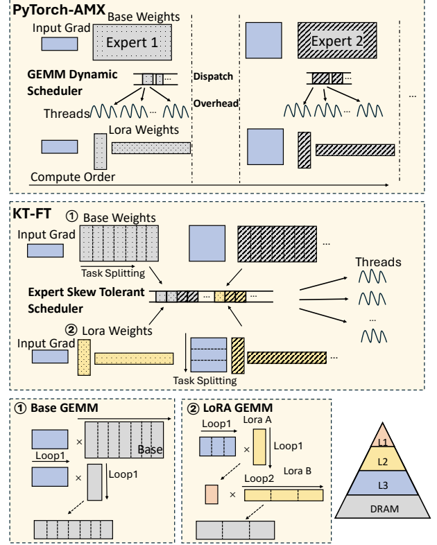
Figure 6. The upper panel shows PyTorch(OneDNN) executing experts sequentially and parallelizing each GEMM across CPU threads. The lower panels show KT-FT’s Skew-Tolerant Dynamic Thread Scheduler dividing base-weight and LoRA computation into a shared pool of tasks according to their memory behavior.
