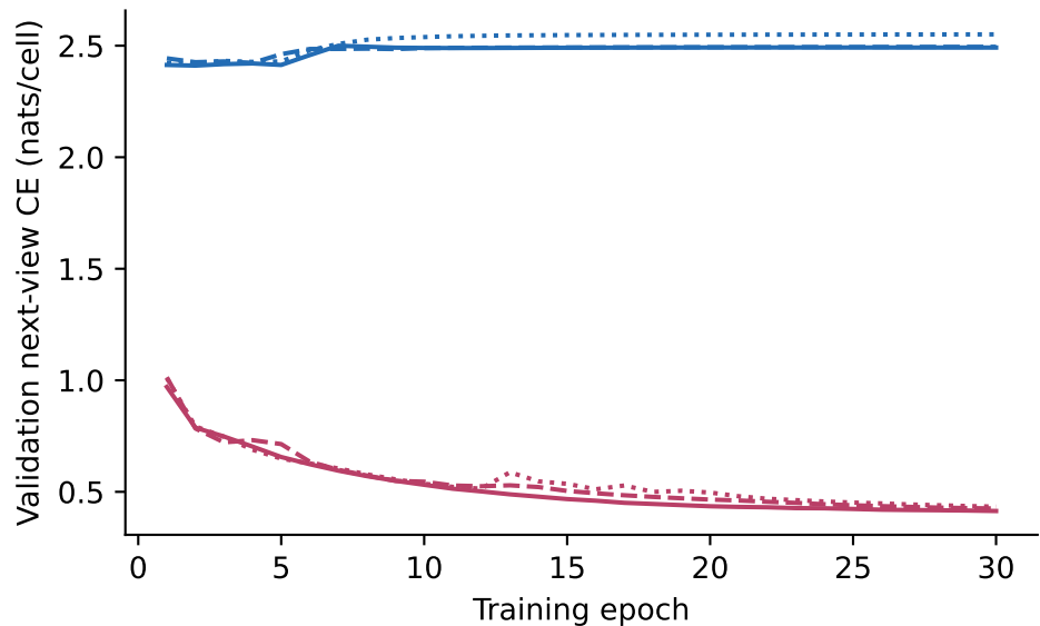
All main training seeds; selection uses validation task CE
