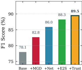
(a) Cumulative Contribution
