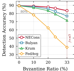
(a) Model Poisoning Attack
