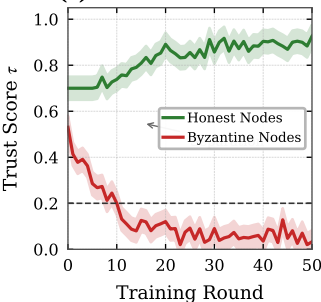
(c) Trust Score Evolution
