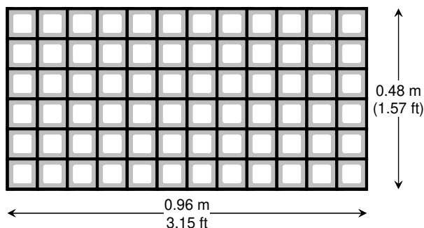
Figure 1 GEOTERRA Unit
