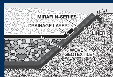
Liner Protection Within a Landfill
