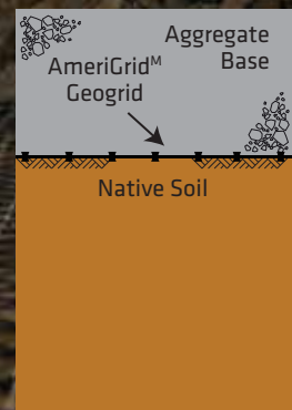
With AmeriGrid Geogrid
