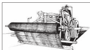
Fabric Tractor†
