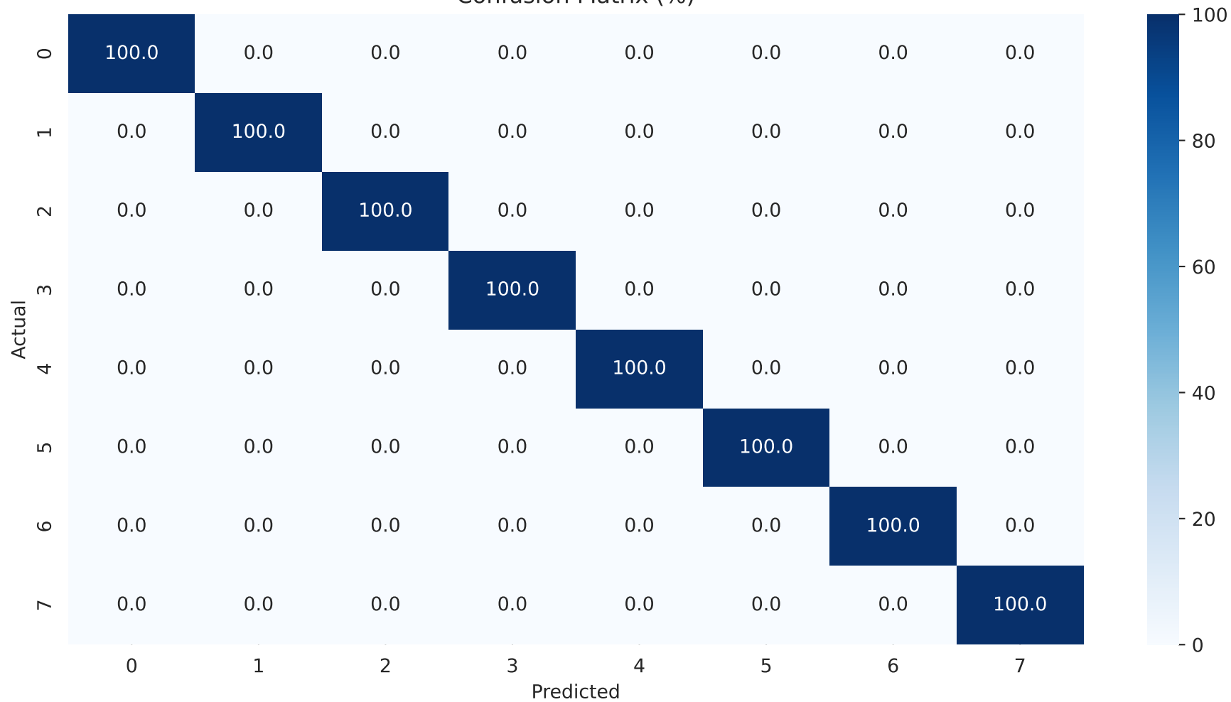
Confusion Matrix (%)
