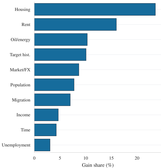
XGBoost feature-group importance
