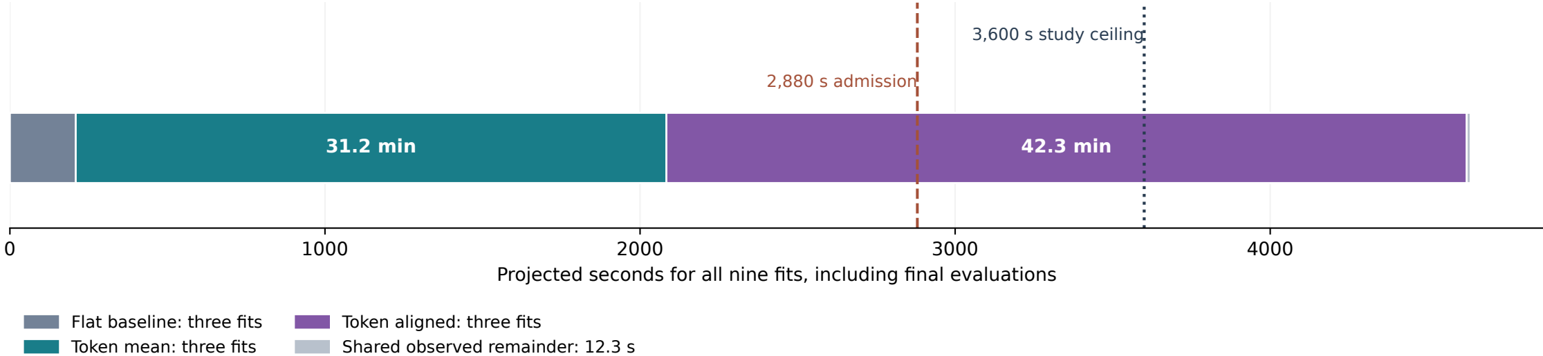
Nine-fit projection: 4,636.0 seconds (77.27 minutes)
