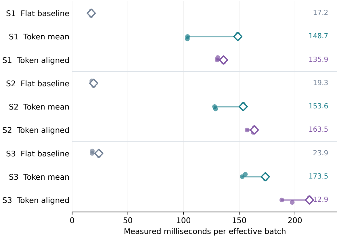
Evaluation: forward + output materialization
