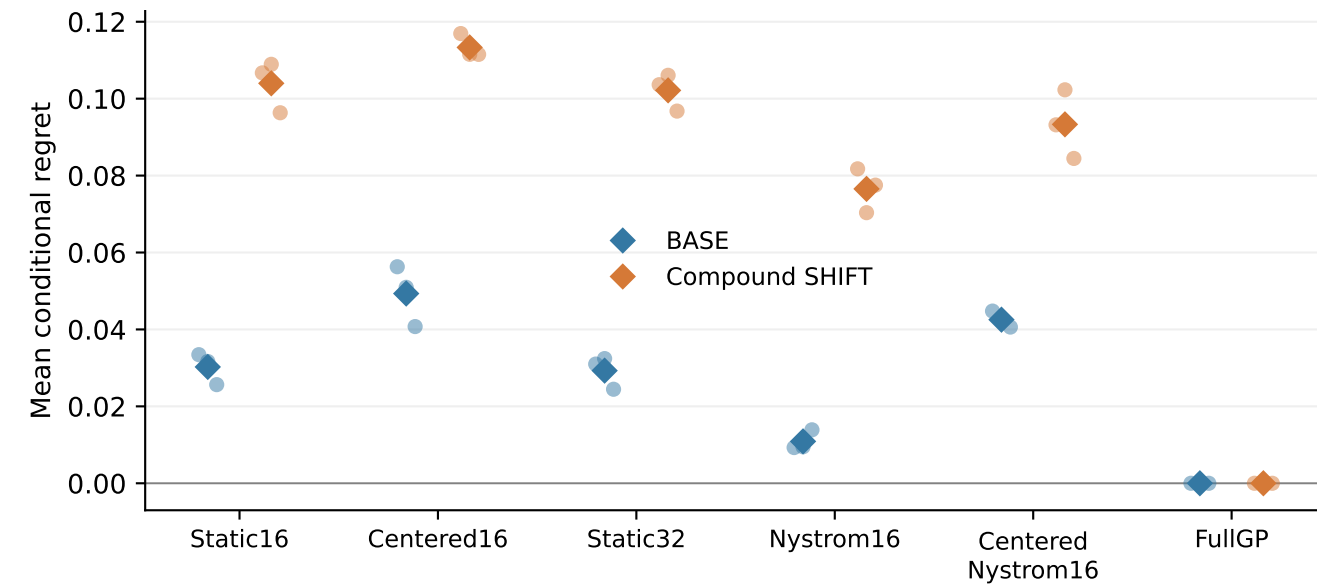
Decision regret under the exact public GP
