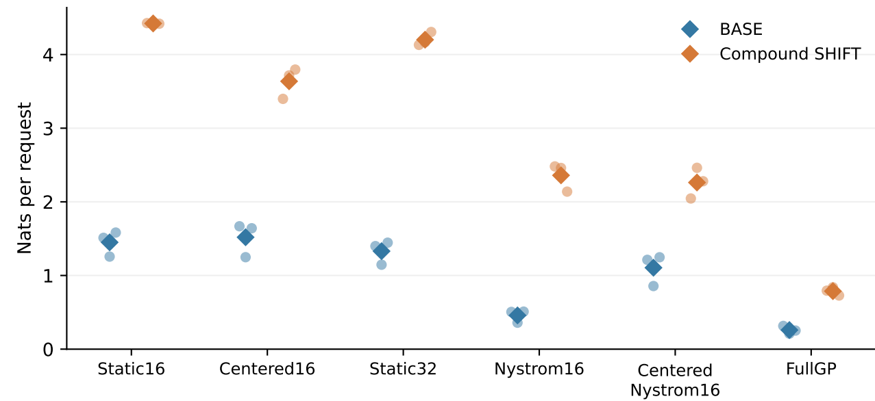
Predictive negative log likelihood
