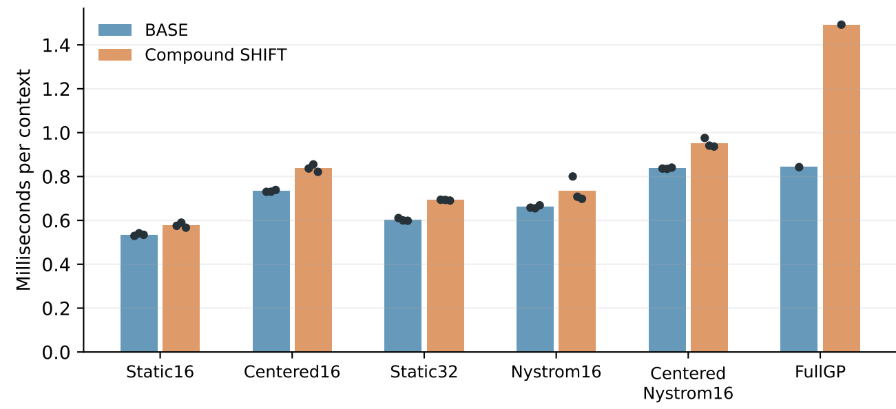
Four-request context latency, including archive work
