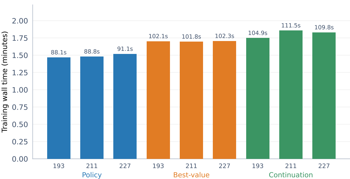
D. Every completed fit: recorded MPS wall time
