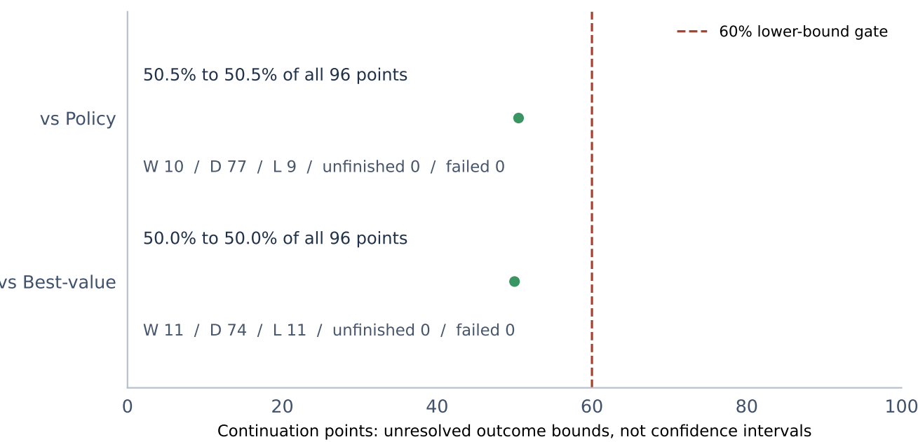
C. Paired games: all 192, actor-only inference
