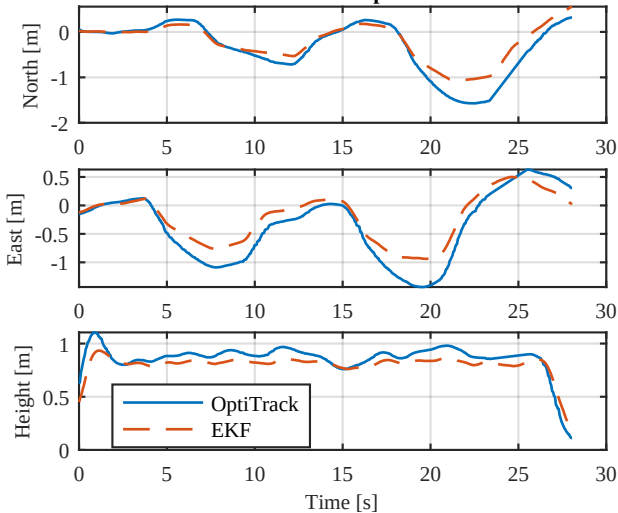
EKF Position Estimate vs OptiTrack Benchmark
