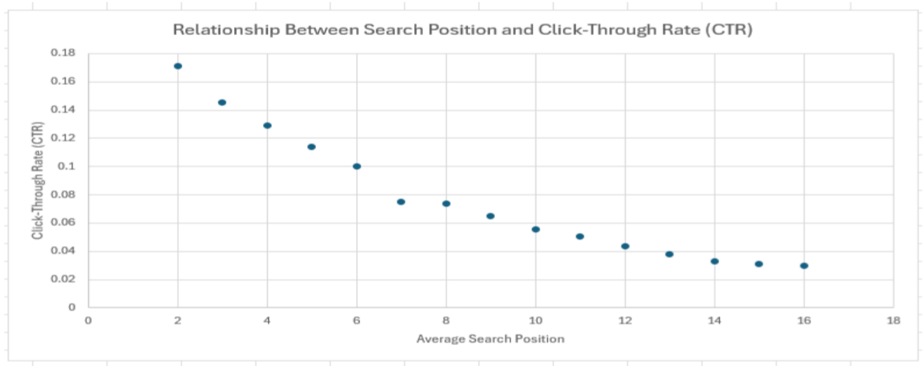
Chart 6: Relationship Between Search Position and Click-Through Rate
