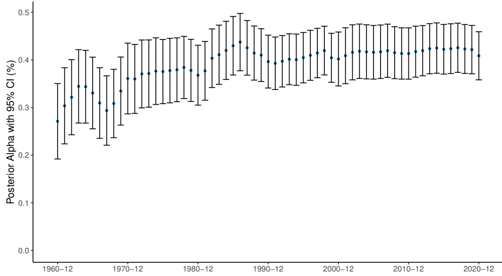
Figure IA.4: World factor alpha posterior distribution over time. The figure reports the CAPM alpha and 95% posterior confidence interval for an equal-weighted portfolio of World factors based on EB posteriors re-estimated in December each year. In contrast to figure 9, we re-estimate \tau_c and \tau_w at each point in time. Figure IA.5 shows how the estimated \tau_c and \tau_w evolve over time.
