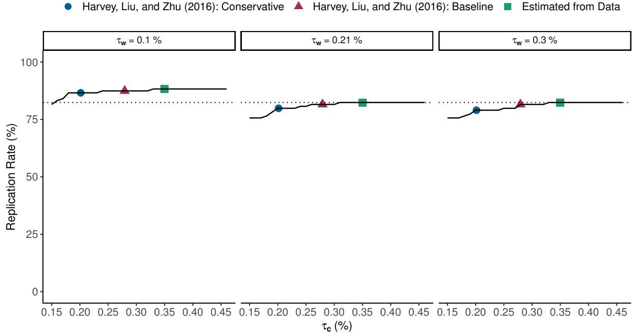
Figure IA.6: Replication rate with prior estimated in light of unobserved factors.
