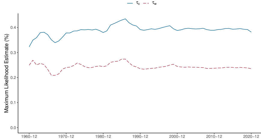
Figure IA.5: World factor hyperparameters over time. The figure reports the \tau_c and \tau_w used in figure IA.4.
