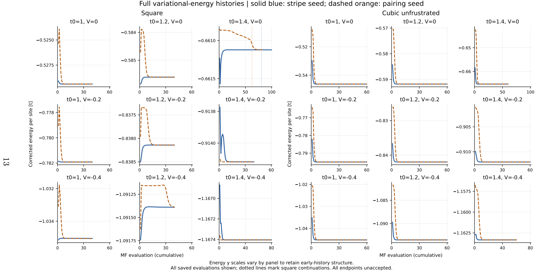
Figure 3: Full target-corrected canonical energy grids, square left and cubic unfrustrated right. Within each geometry, columns are t_0 = 1, 1.2, 1.4 and rows are V = 0, -0.2, -0.4 . Solid blue and dashed orange denote stripe and pairing seeds. All 902 square and 1080 cubic saved evaluations are included. Dotted lines mark the square continuations after evaluations 80 and 62; curves end at their own final evaluations. Matching coordinates share an iteration range, while energy y scales vary by panel.
