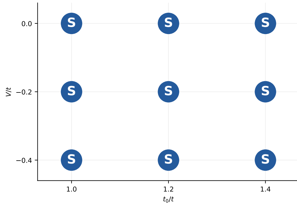
Cubic unfrustrated
