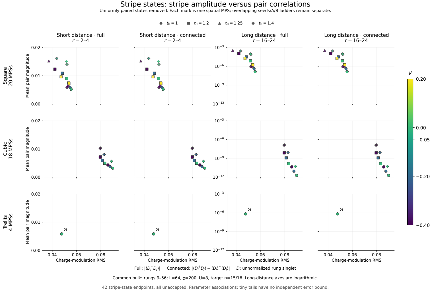
Figure 19: Pair correlations versus static charge RMS in the 42 stripe-state MPSs, with all uniformly paired states removed. Rows separate square, cubic and trellis geometries; columns separate short/long distances and full/connected correlations. Color denotes V and marker shape t_0 . Definitions and analysis are in Section 3.15. All endpoints remain unaccepted; overlapping seeds and A/B ladders are retained.
