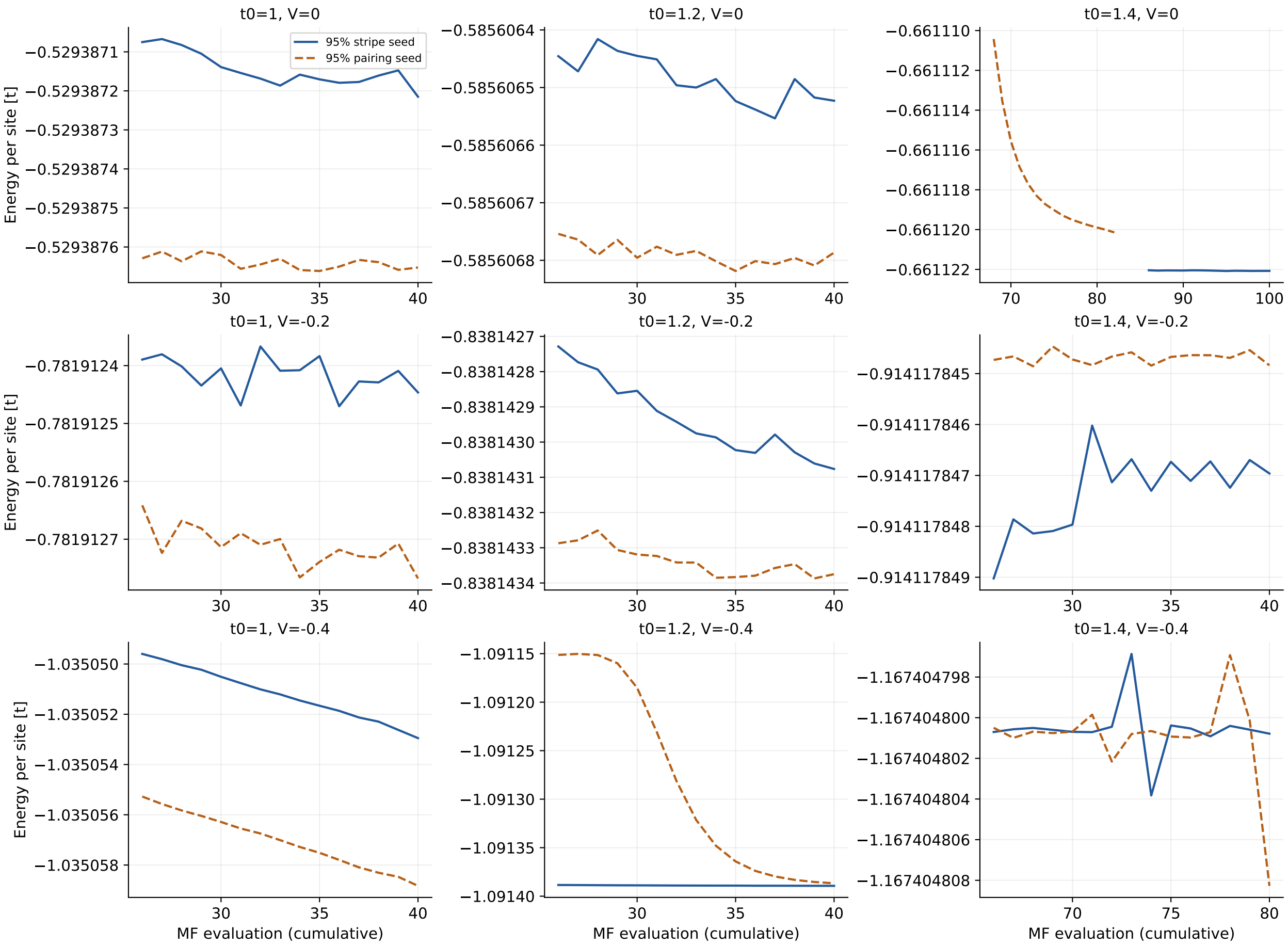
Corrected canonical energy: final 15 evaluations Square grid; solid = stripe seed, dashed = pairing seed; no accepted endpoints
