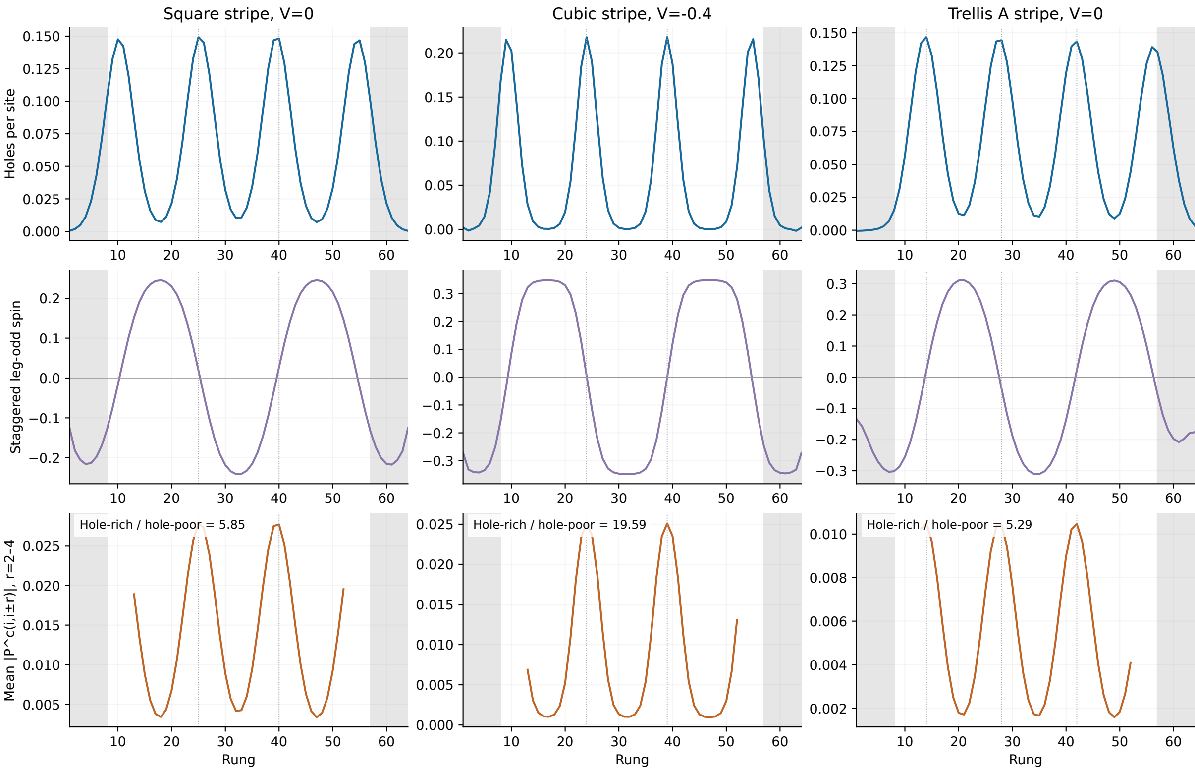
Short-distance pair correlations and stripe texture Dotted lines: interior hole-density maxima; shading: excluded edge rungs
