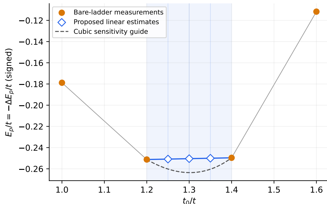
Bare pair binding; V/t = -0.4
