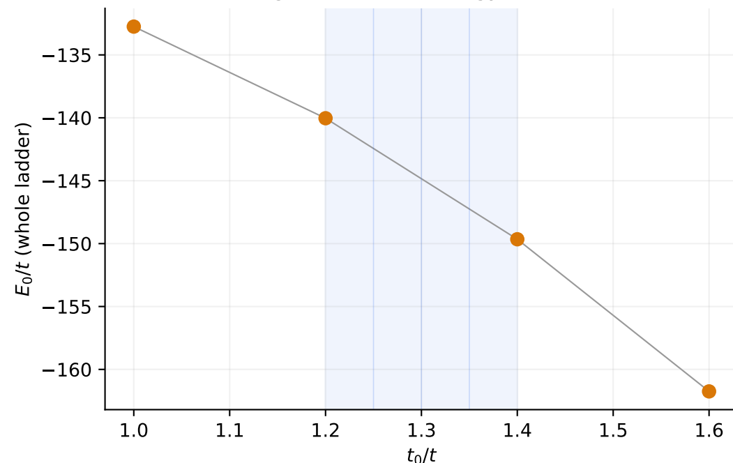
Bare ground-state energy; V/t = -0.4
