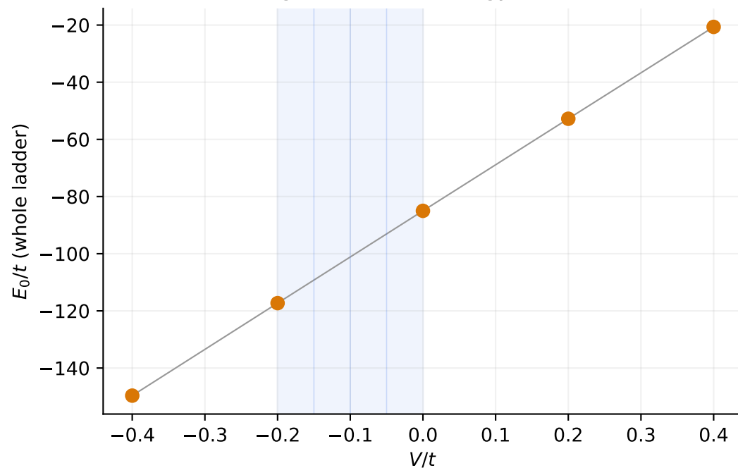
Bare ground-state energy; t_0/t = 1.4
