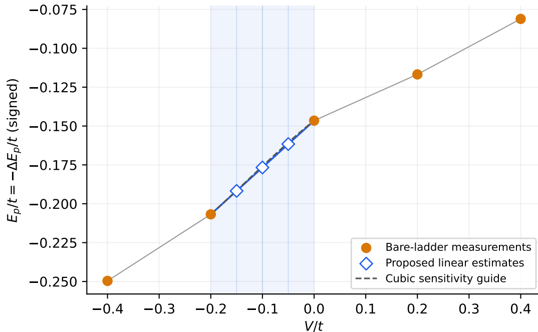
Bare pair binding; t_0/t = 1.4
