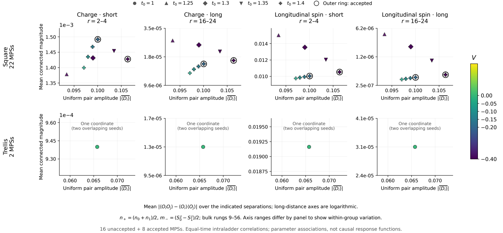
Figure 20: Short- and long-distance connected charge and longitudinal-spin magnitudes versus uniform pairing in the same 24 MPSs. Both rungs lie in 9–56; each panel averages |C_O(i, j)| over its indicated separation window. Contact terms are excluded, and the long-distance axes are logarithmic. These spatial measures are not restricted to a stripe wavevector. Marker conventions match Fig. 19; the opposite trends along the two square parameter cuts remain visible.
