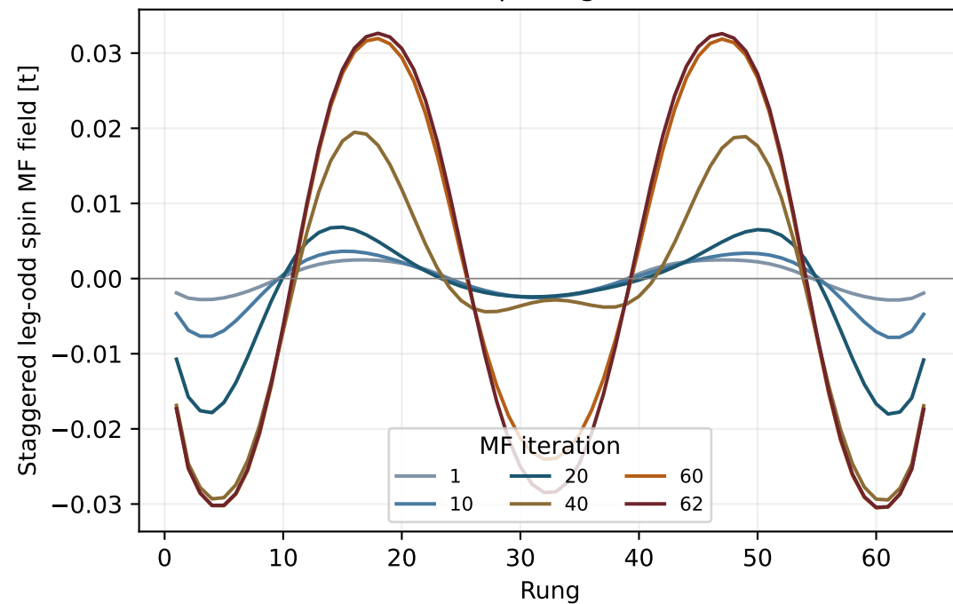
95% pairing seed
