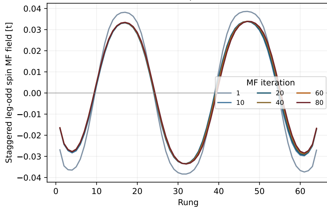
95% stripe seed
