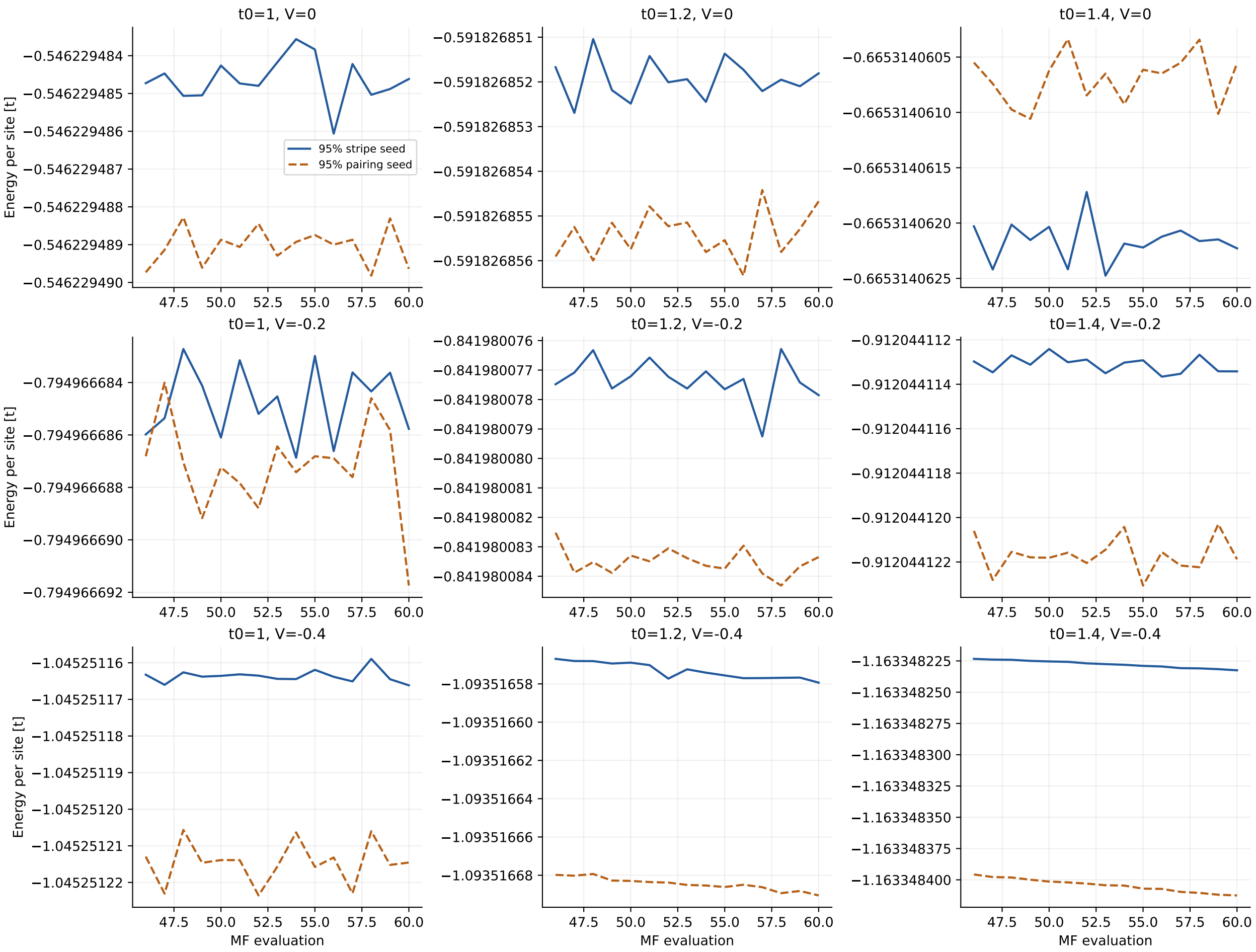
Corrected canonical energy: final 15 evaluations Cubic unfrustrated; solid = stripe seed, dashed = pairing seed; no accepted endpoints
