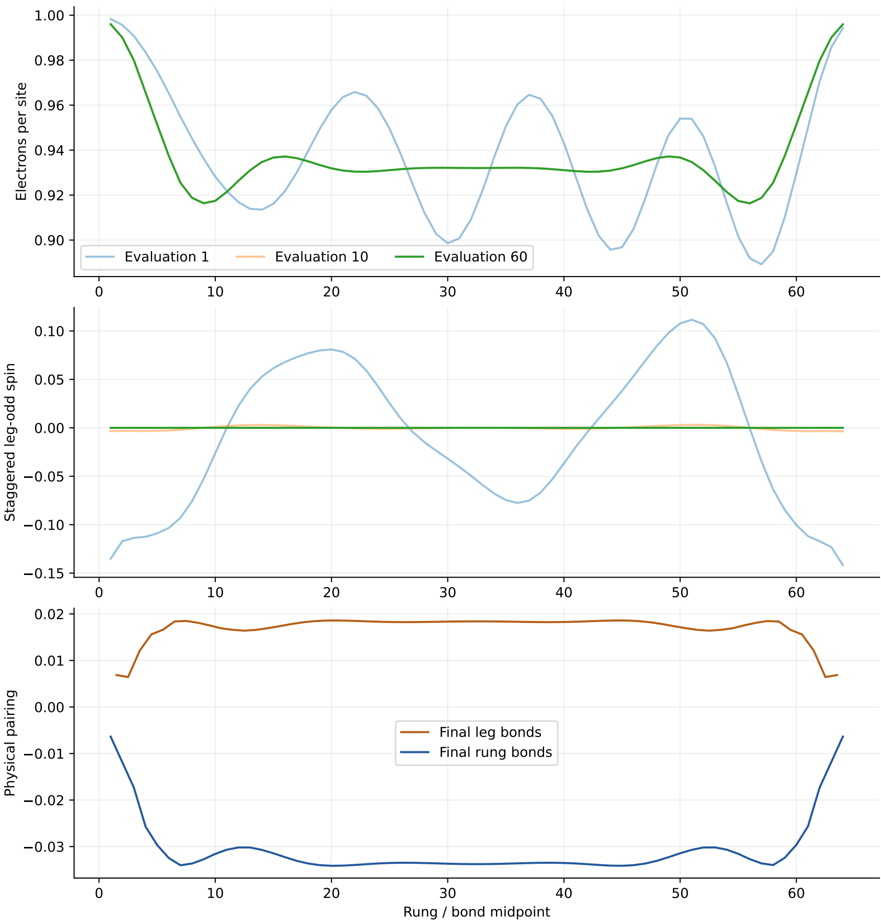
Trellis: spin texture disappears, opposite leg/rung pairing survives
