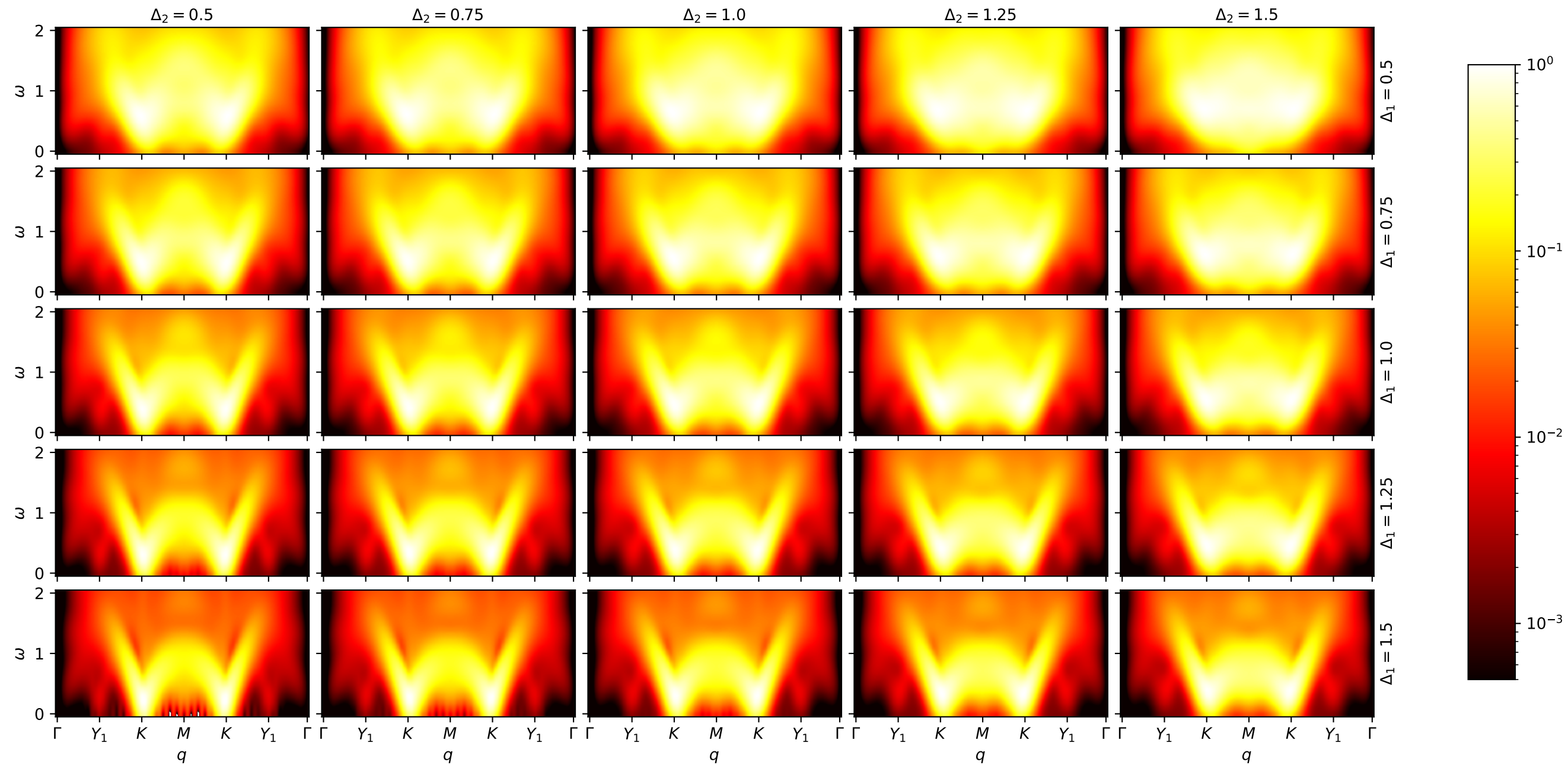
S(q, \omega)/S_{\max} for J_2 = 0.072 and varying XXZ anisotropies
