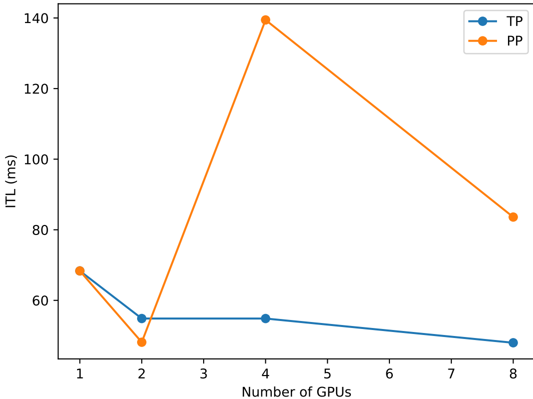
ITL vs Number of GPUs for 8b model
