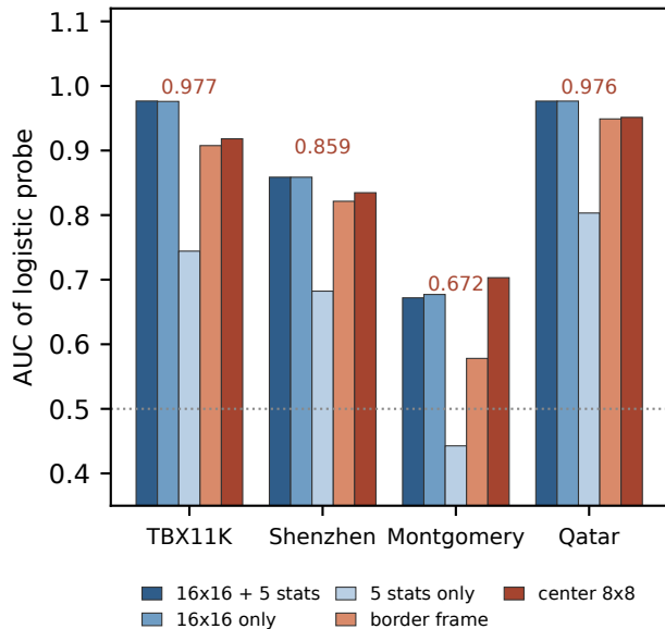
(b) Low-level reference, same splits
