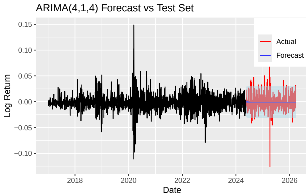
Figure 10: ARIMA(4,1,4) Forecast Data Compared with Actual Data
