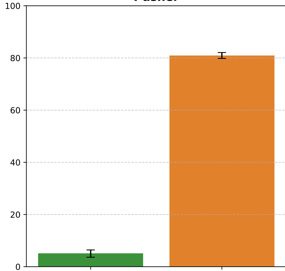
Pusher
