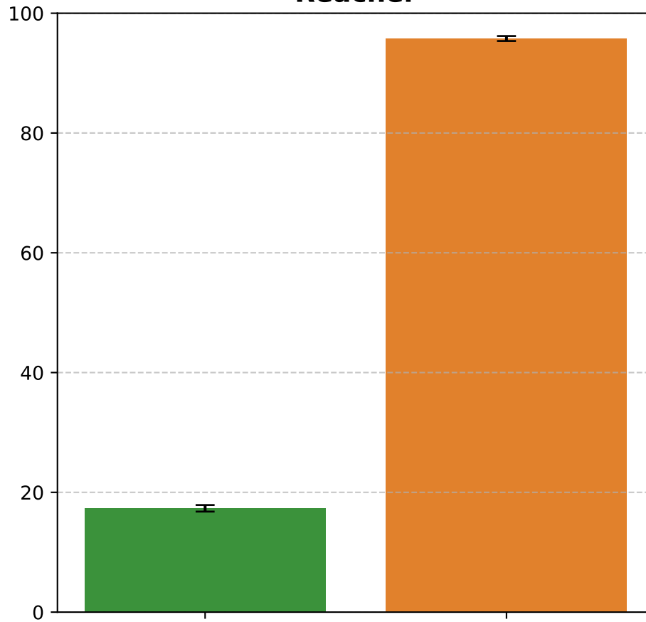
Reacher
