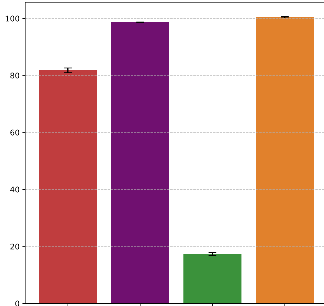
Reacher
