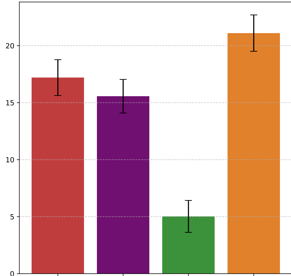
Pusher
