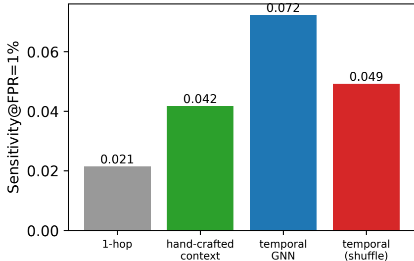
Sensitivity at FPR=1%
