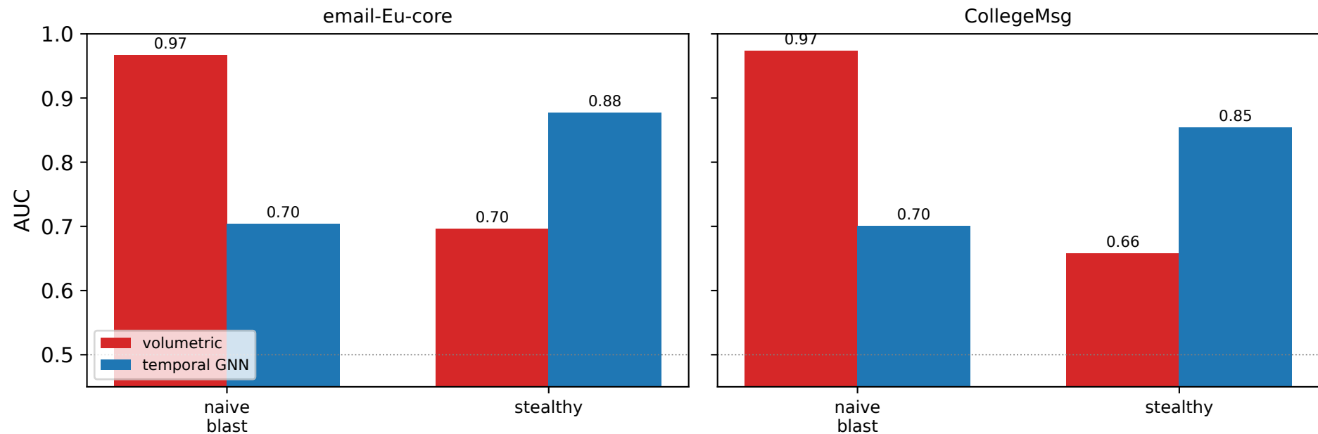
Real topologies: volumetric wins the blast, collapses under the stealthy attacker; temporal GNN maintains the advantage
