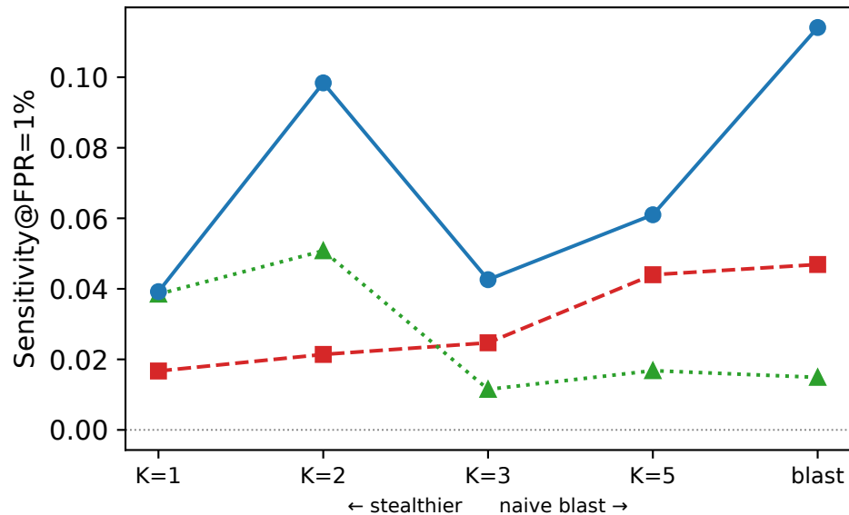
Sensitivity@FPR=1%
