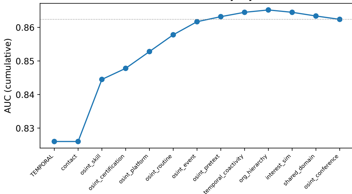
Forward selection: how many layers suffice
