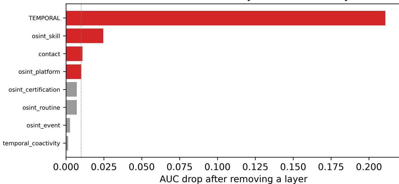
Leave-one-out: which layers are necessary
