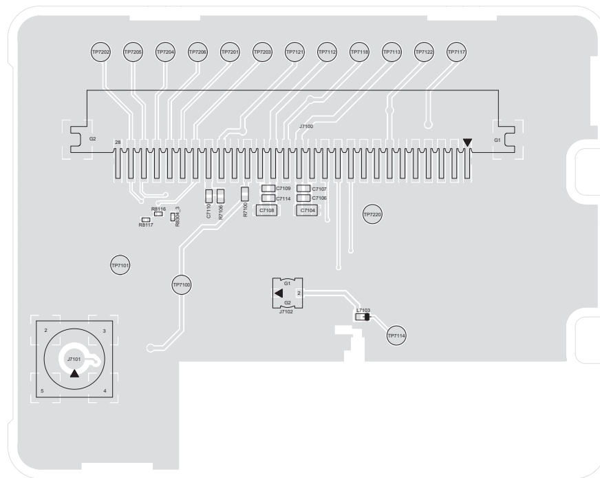
Bluetooth/Wi-Fi/GNSS (PMLN7252_S) Expansion Board – PCB PC000942A01-AA Bottom Side
