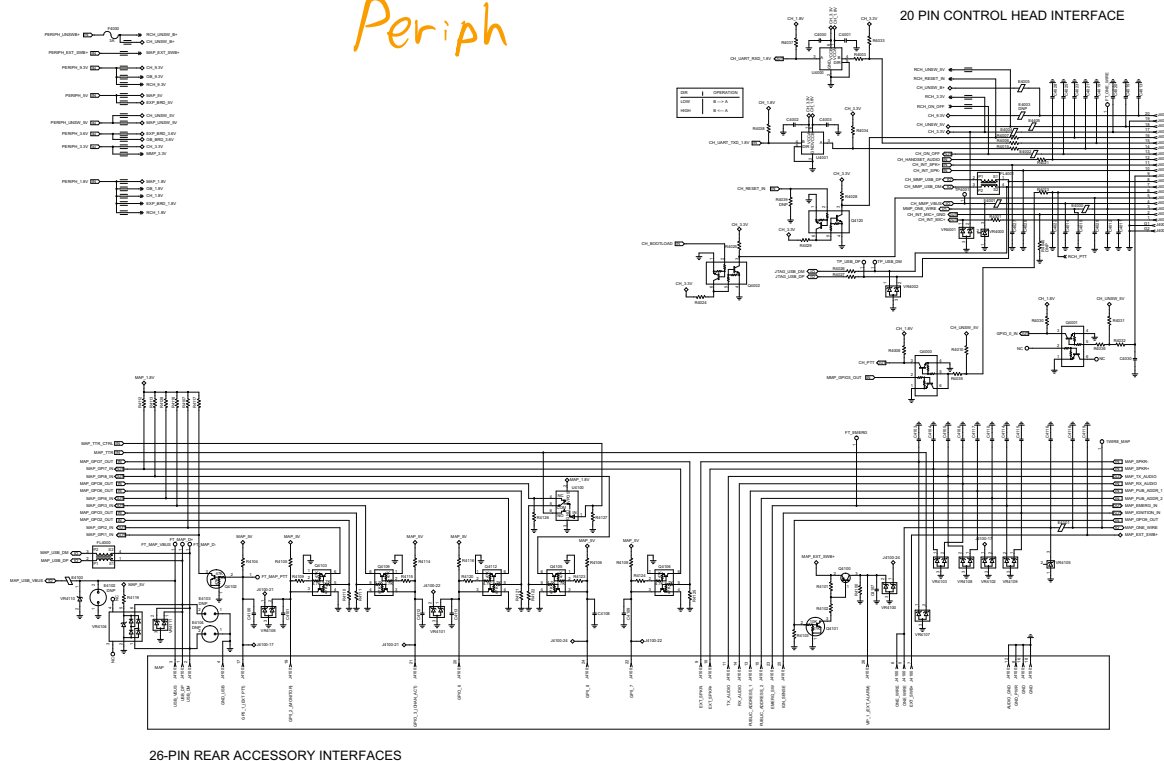
Controller Peripheral Schematic Diagram (sheet 1 of 2)
