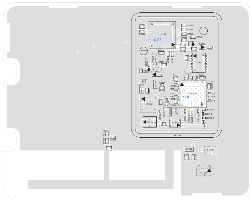
Bluetooth/Wi-Fi/GNSS (PMLN7252_S) Expansion Board – PCB PC000942A01-AA Top Side
