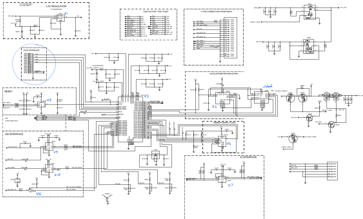
GOB Schematic Diagram
