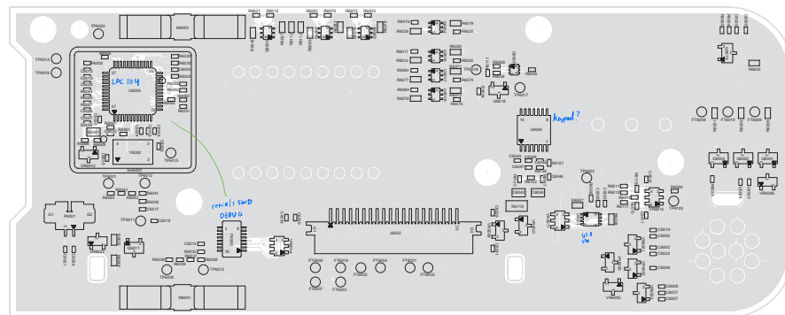
Bottom Side View
