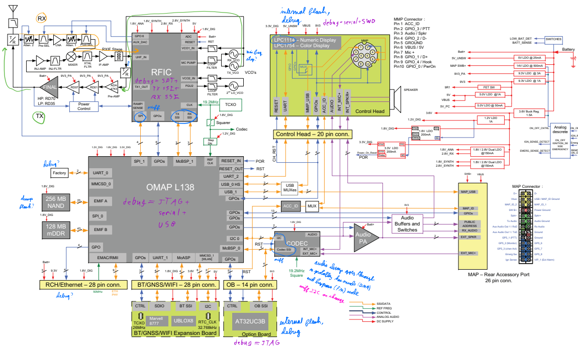
Figure 1-1 Top Level Block Diagram (for PCB PC000942A01-AA)
