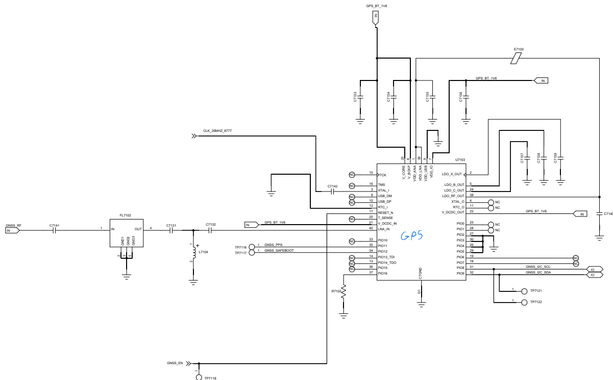
Bluetooth/Wi-Fi/GNSS (PMLN7252_S) Expansion Board Schematic Diagram (sheet 2 of 4)
