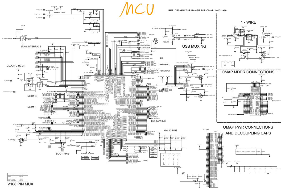
Controller Microprocessor Schematic Diagram
