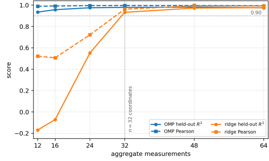
Figure 2: Aggregate recovery of the 32-coordinate finite-effect map. OMP scores Pearson r = 0.989 and held-out R^2 = 0.935 with 12 aggregate measurements. Ridge gives comparable held-out prediction with 32 measurements, the exhaustive coordinate count.
