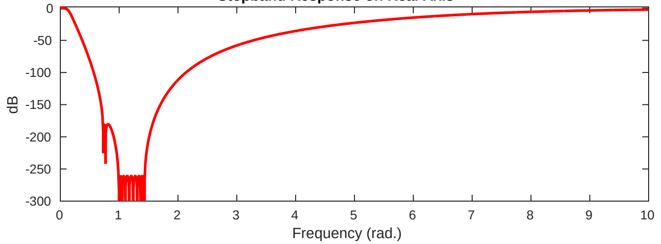
Stopband Response on Real Axis
