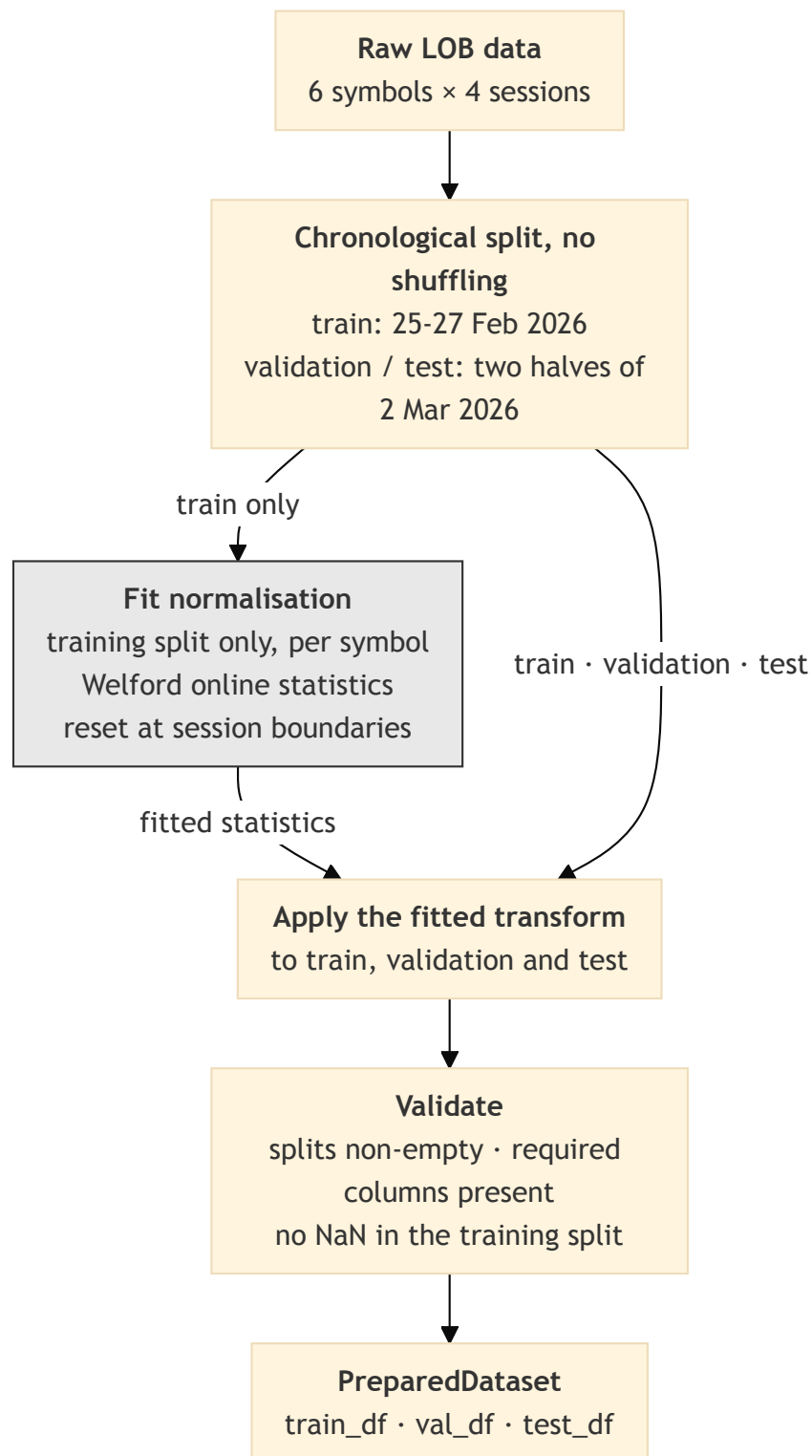
Fig. 6. Data preparation pipeline.
